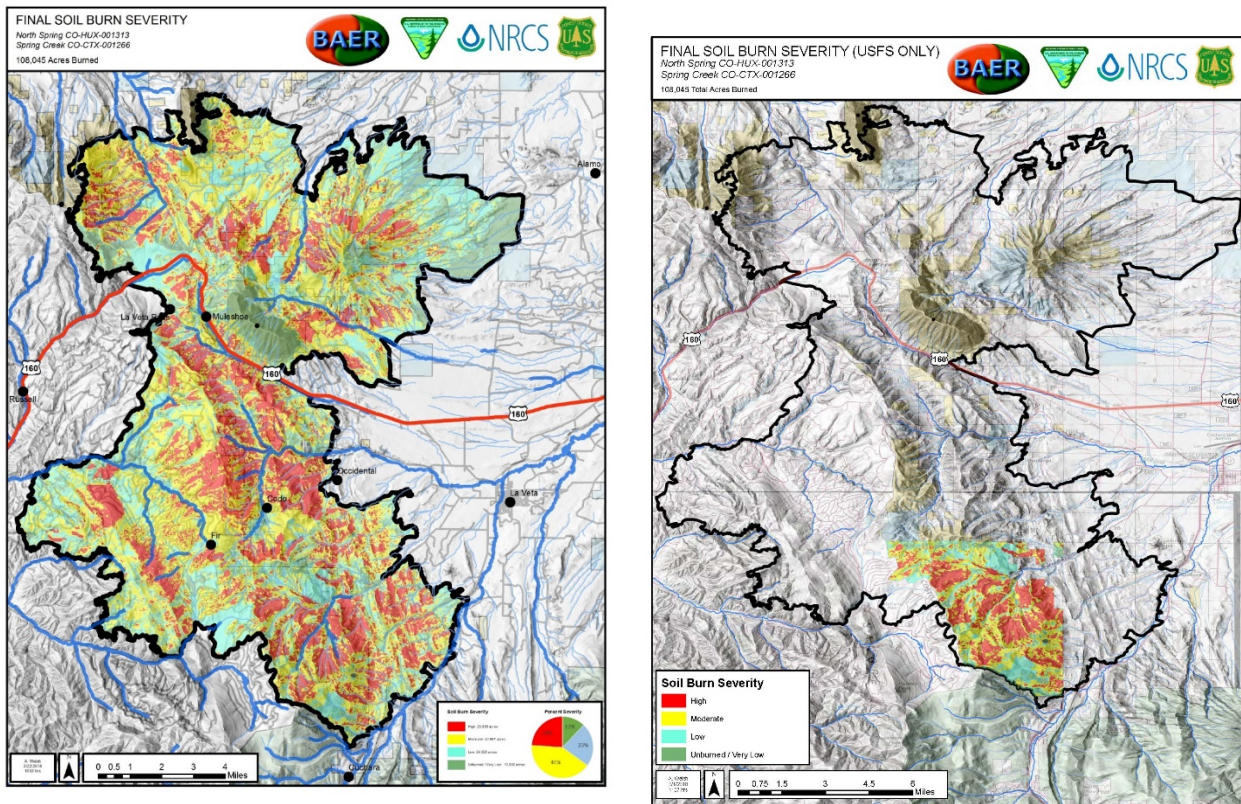
Map 1.1: Soil Burn Severity (Forest only)
