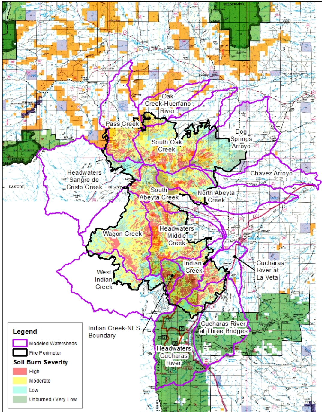
Map 3: Modeled Hydrologic Units for the Spring Fire.
