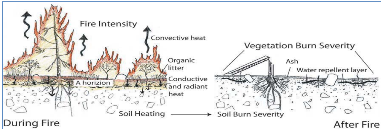
Figure 1: Effect of Fire Intensity on Above-ground Vegetation and Below-ground Soil Properties (Graphics by Mike Hankinson, National Park Service)
