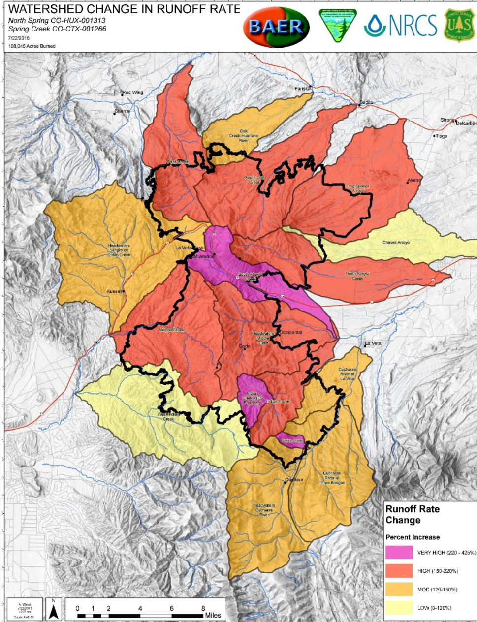
Map 4: Magnitude of Post-fire Runoff Within the Modeled Watersheds.
